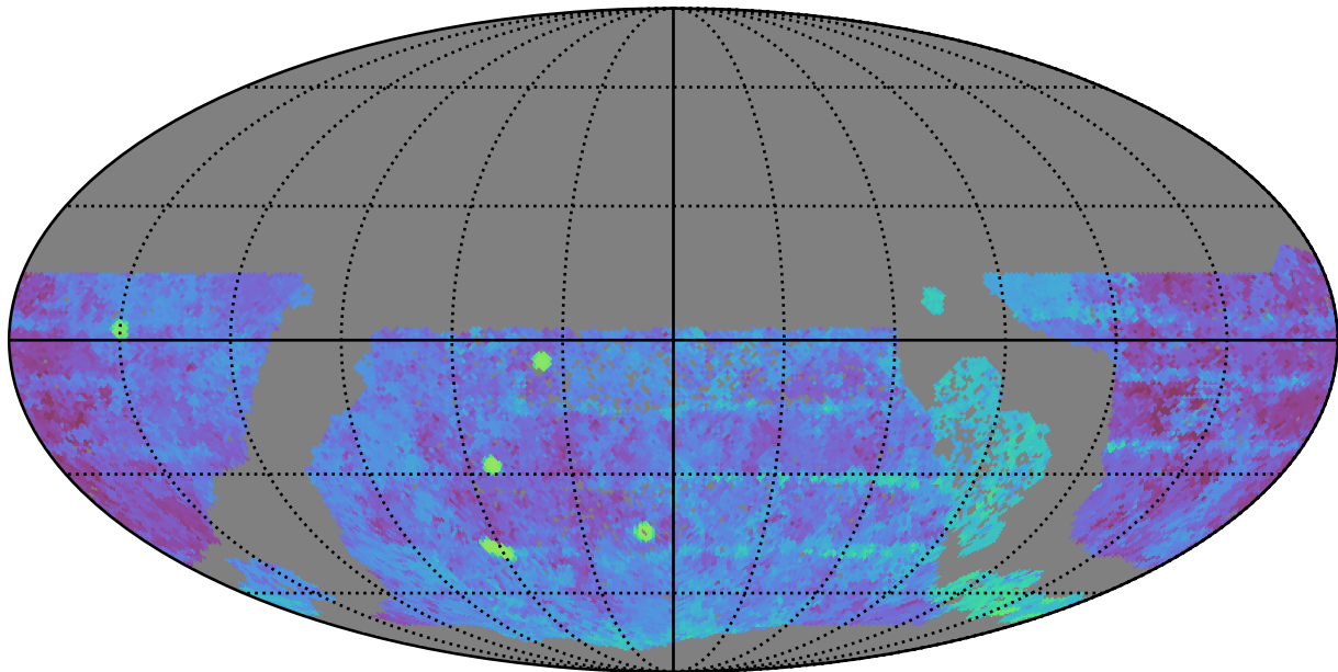
ddf_half_v3.4_10yrs WFD g band: Median Season Length
