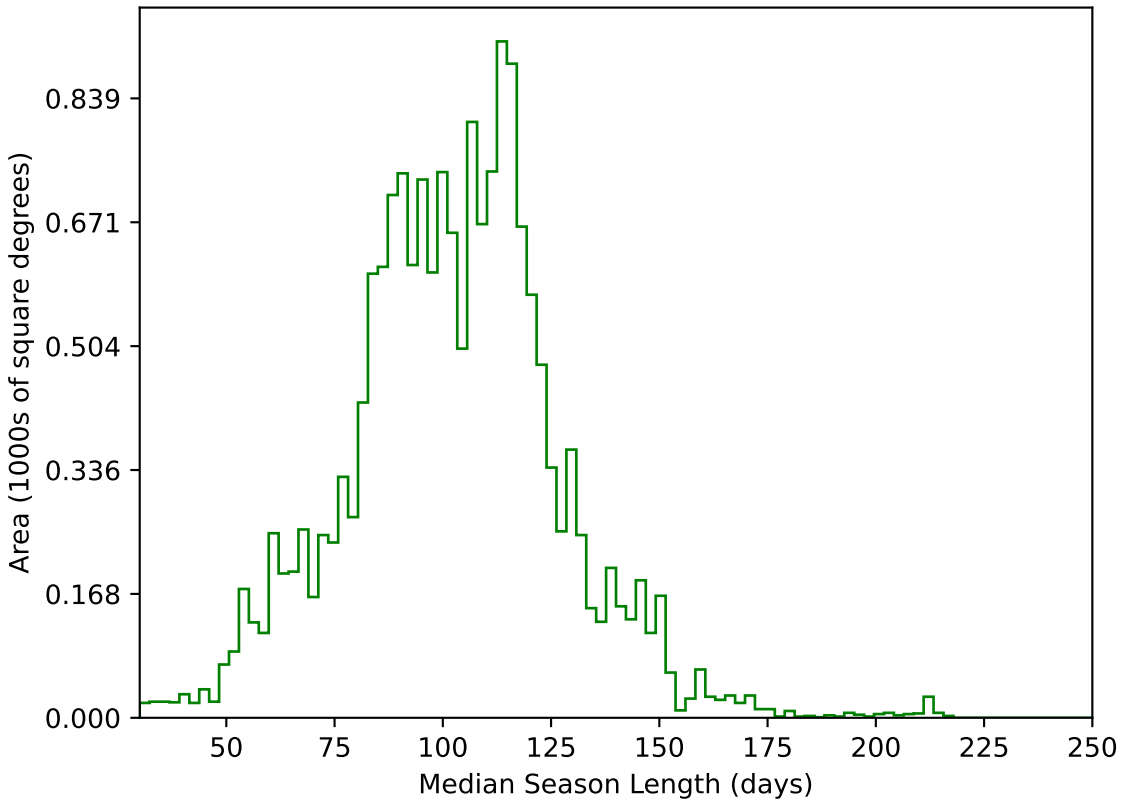
ddf_half_v3.4_10yrs WFD g band: Median Season Length
