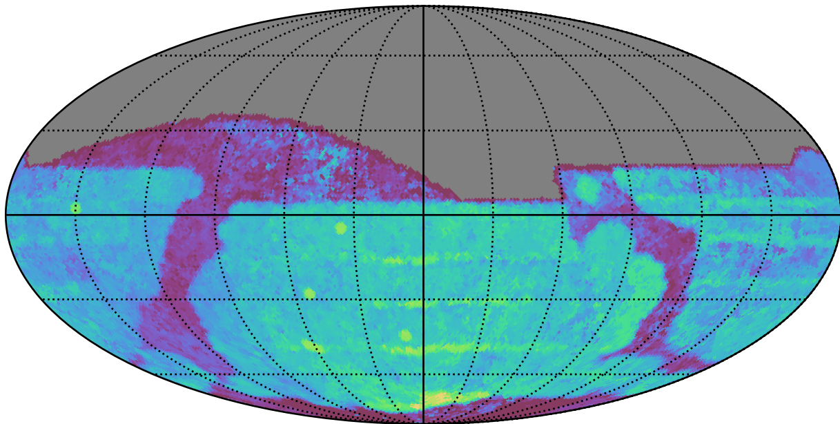
ddf_half_v3.4_10yrs All sky z band: Median Season Length
