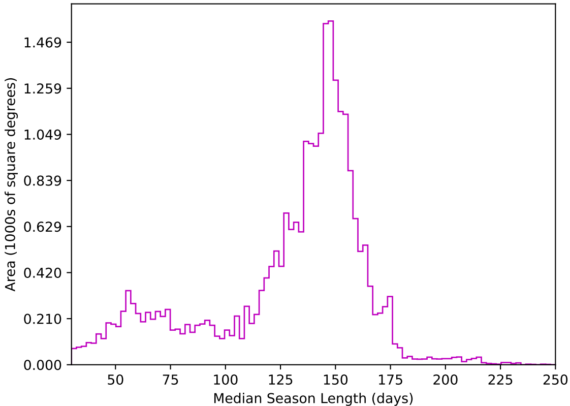
ddf_half_v3.4_10yrs All sky z band: Median Season Length
