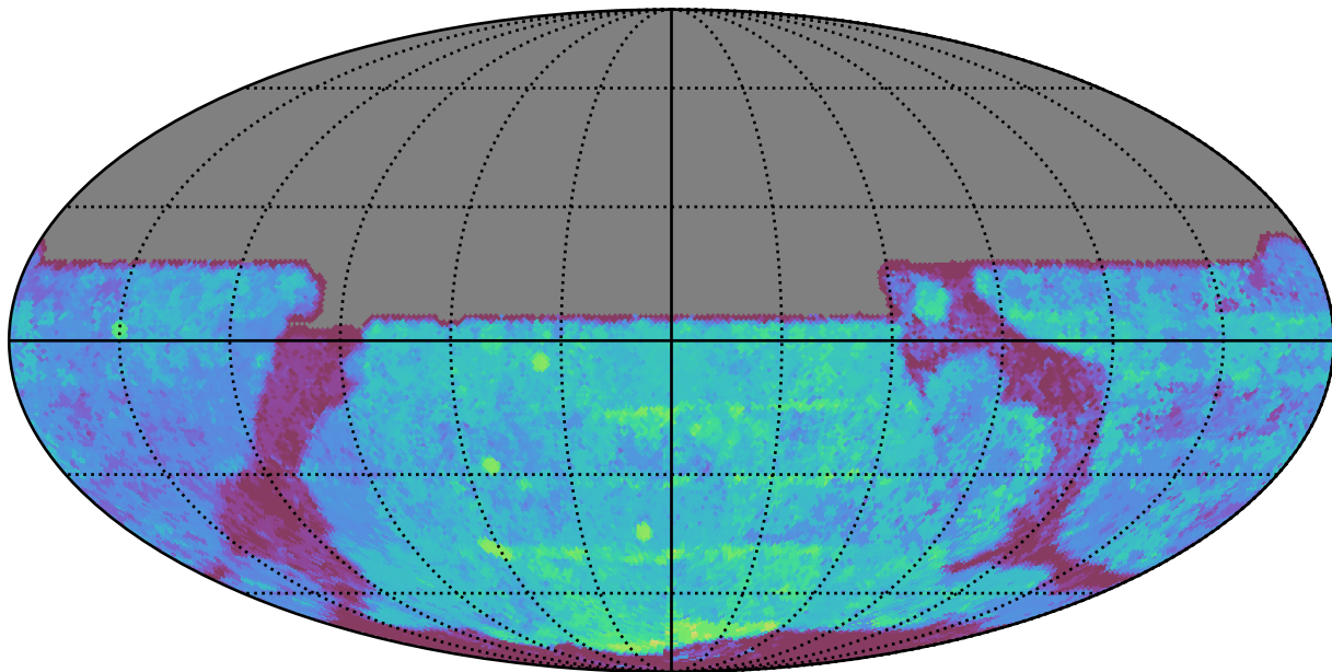
ddf_half_v3.4_10yrs All sky y band: Median Season Length
