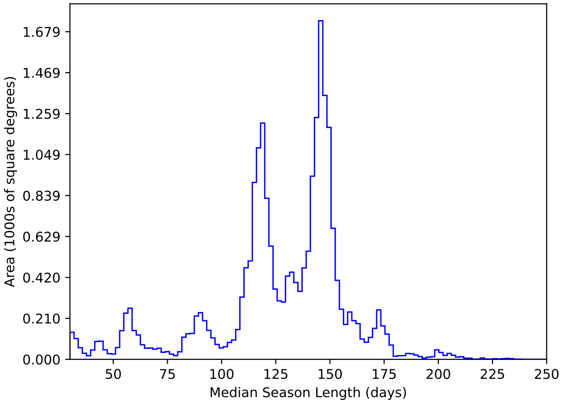
ddf_half_v3.4_10yrs All sky y band: Median Season Length
