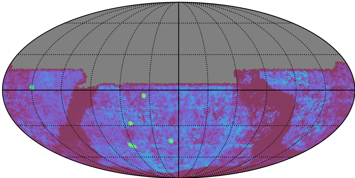
ddf_half_v3.4_10yrs All sky u band: Median Season Length
