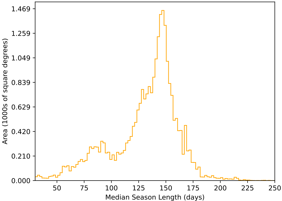
ddf_half_v3.4_10yrs All sky r band: Median Season Length
