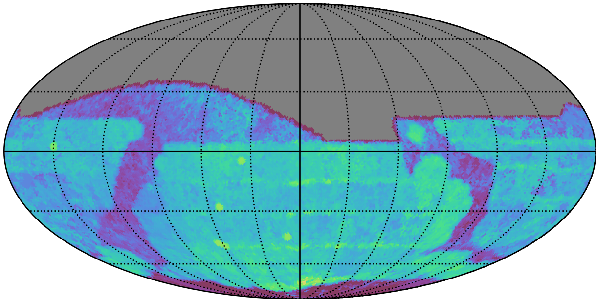
ddf_half_v3.4_10yrs All sky i band: Median Season Length
