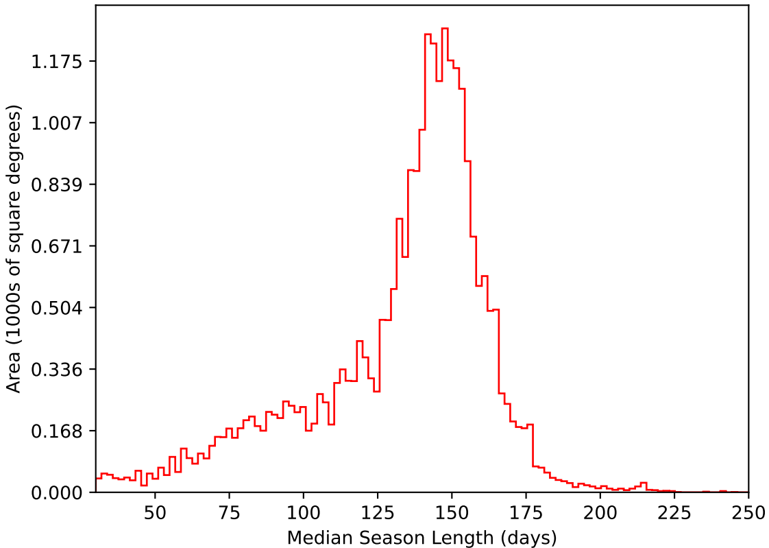
ddf_half_v3.4_10yrs All sky i band: Median Season Length
