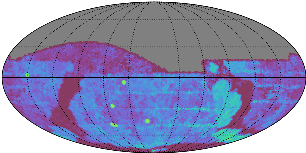
ddf_half_v3.4_10yrs All sky g band: Median Season Length
