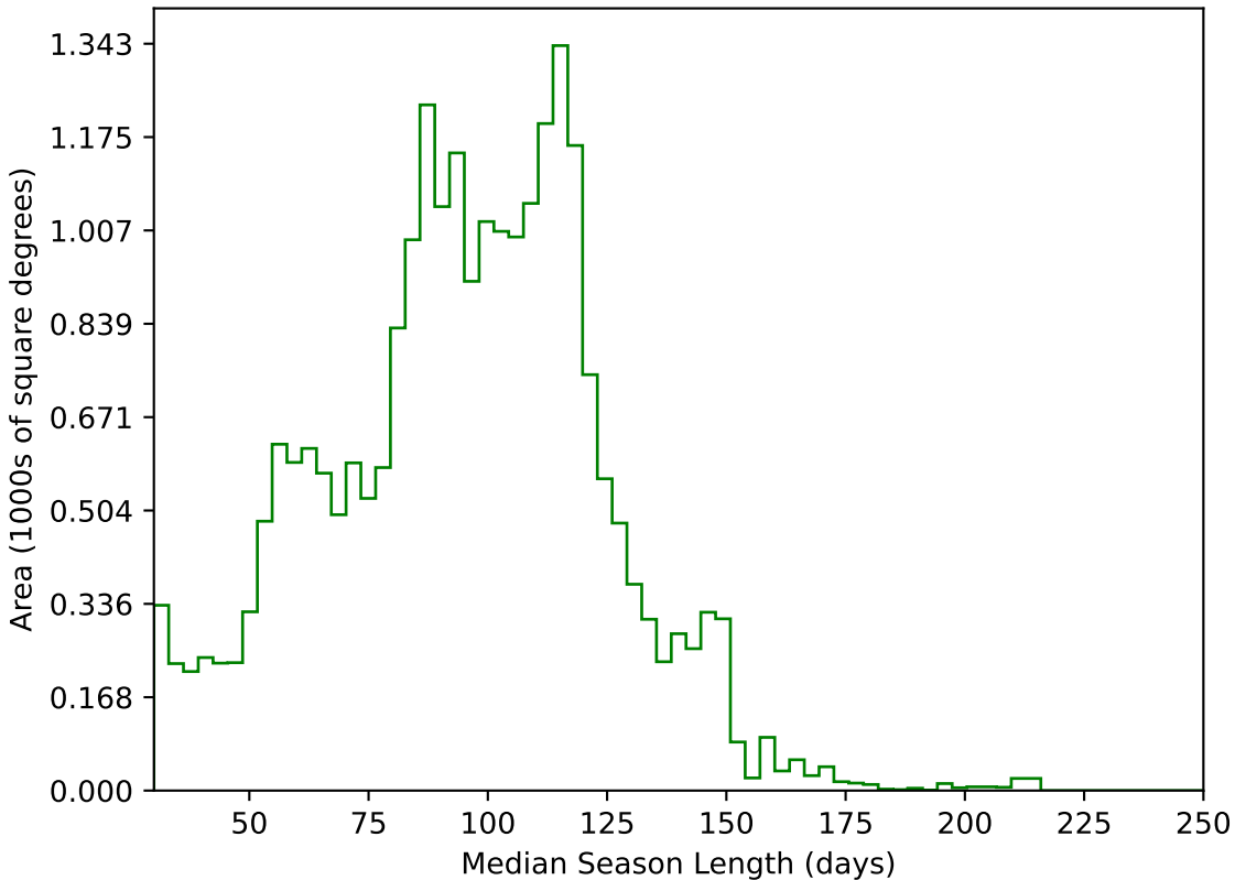
ddf_half_v3.4_10yrs All sky g band: Median Season Length
