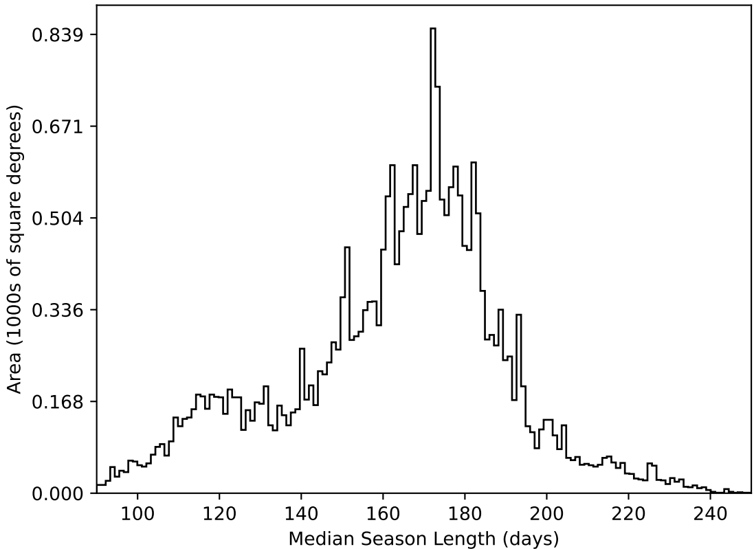
ddf_half_v3.4_10yrs All sky all bands: Median Season Length
