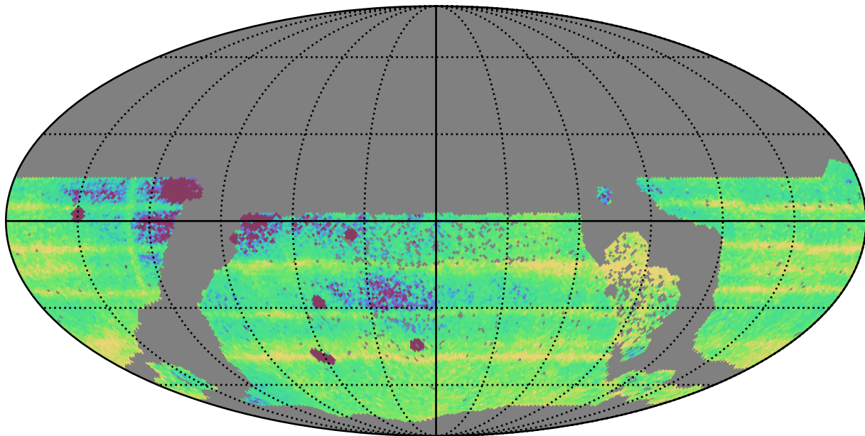
ddf_half_v3.4_10yrs WFD: Median Intra-Night Gap
