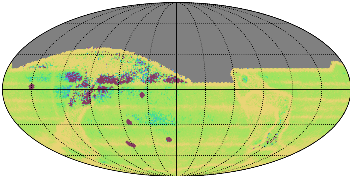
ddf_half_v3.4_10yrs All sky: Median Intra-Night Gap
