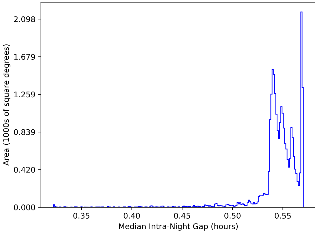
ddf_half_v3.4_10yrs All sky: Median Intra-Night Gap
