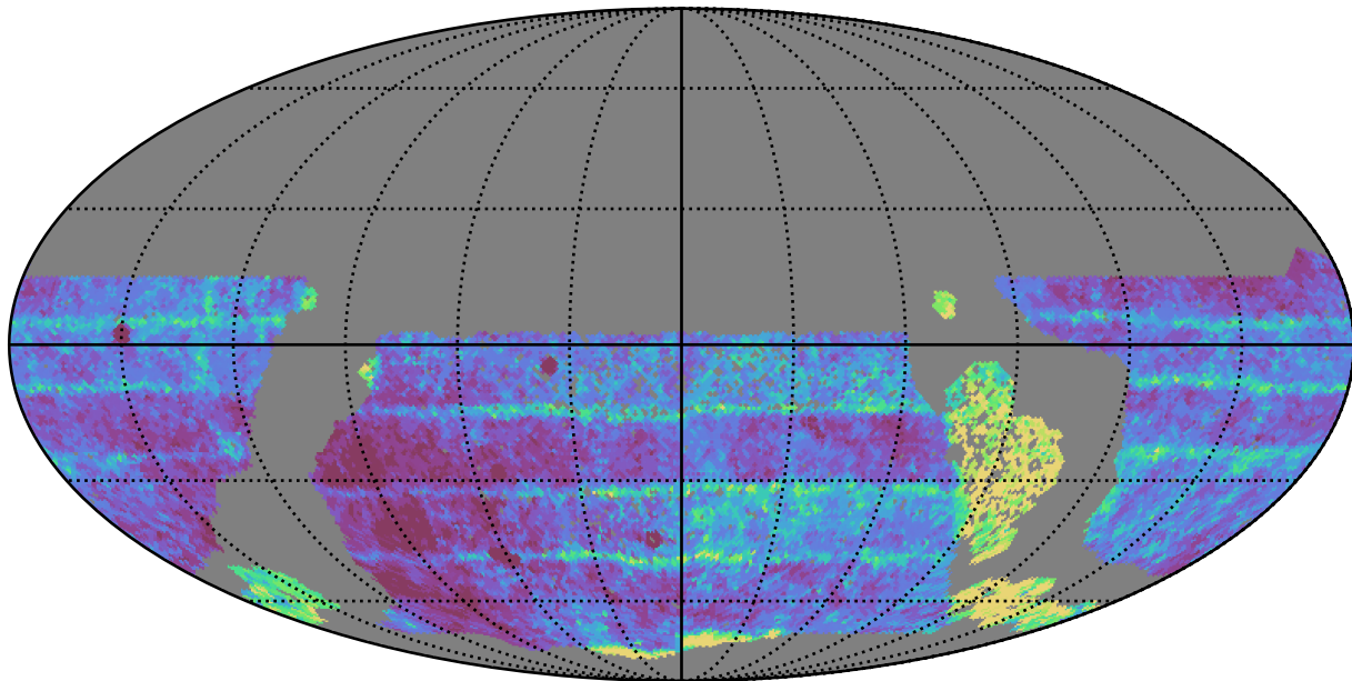
ddf_half_v3.4_10yrs WFD z band: Median Inter-Night Gap
