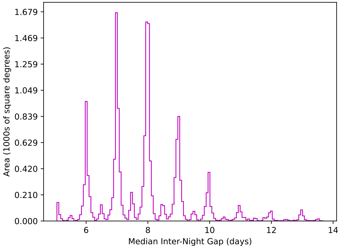
ddf_half_v3.4_10yrs WFD z band: Median Inter-Night Gap
