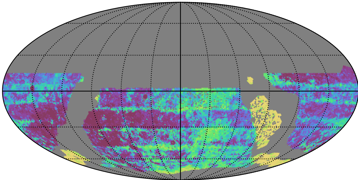
ddf_half_v3.4_10yrs WFD y band: Median Inter-Night Gap
