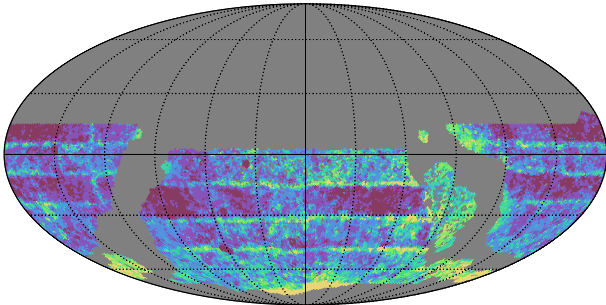
ddf_half_v3.4_10yrs WFD r band: Median Inter-Night Gap
