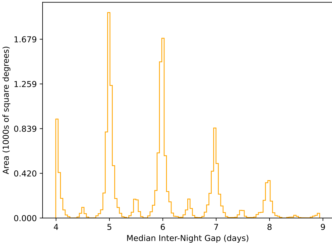
ddf_half_v3.4_10yrs WFD r band: Median Inter-Night Gap
