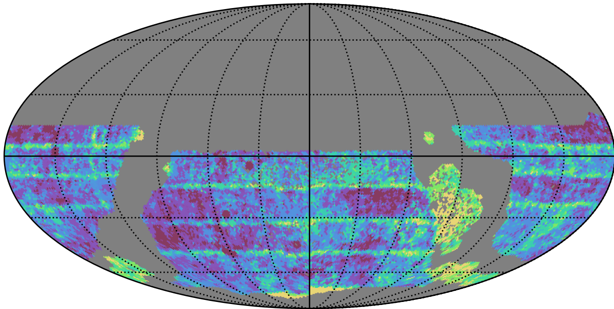
ddf_half_v3.4_10yrs WFD i band: Median Inter-Night Gap
