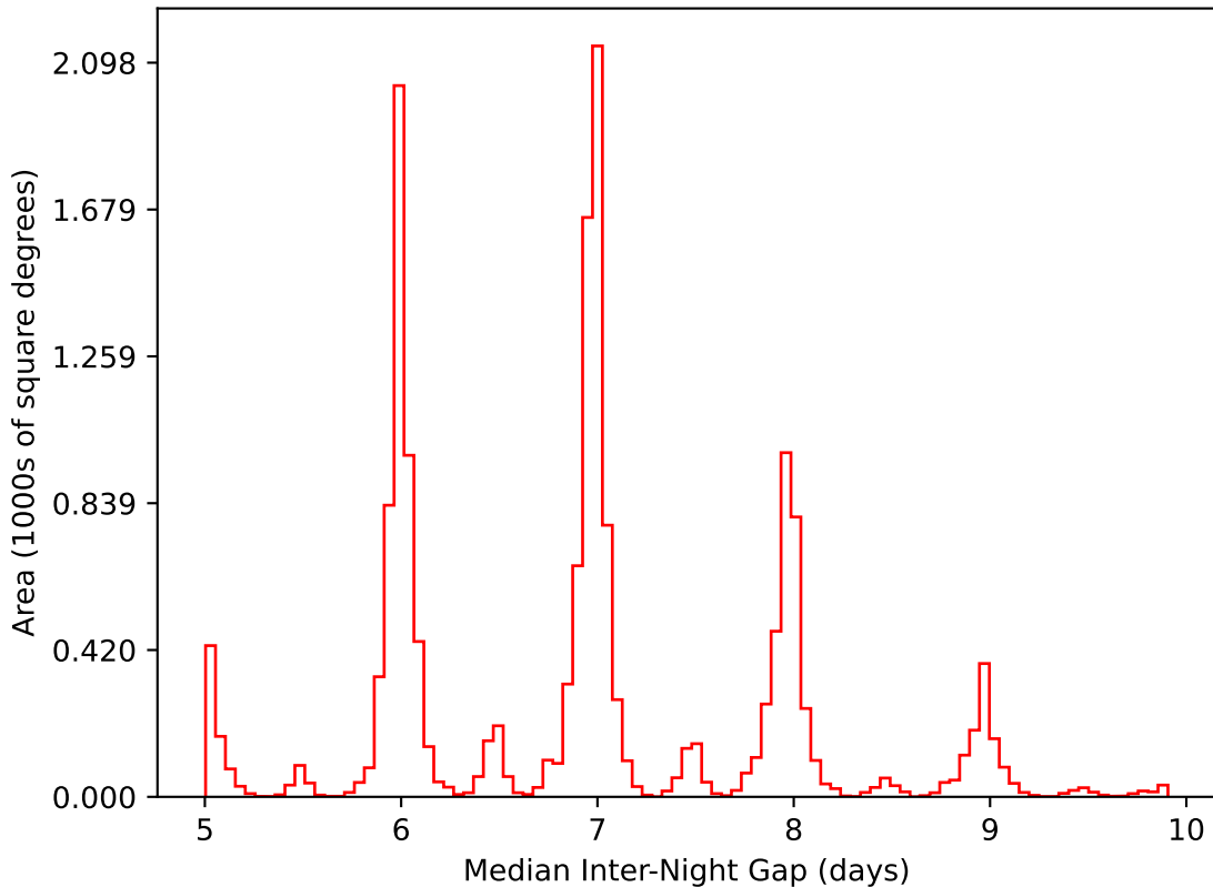
ddf_half_v3.4_10yrs WFD i band: Median Inter-Night Gap
