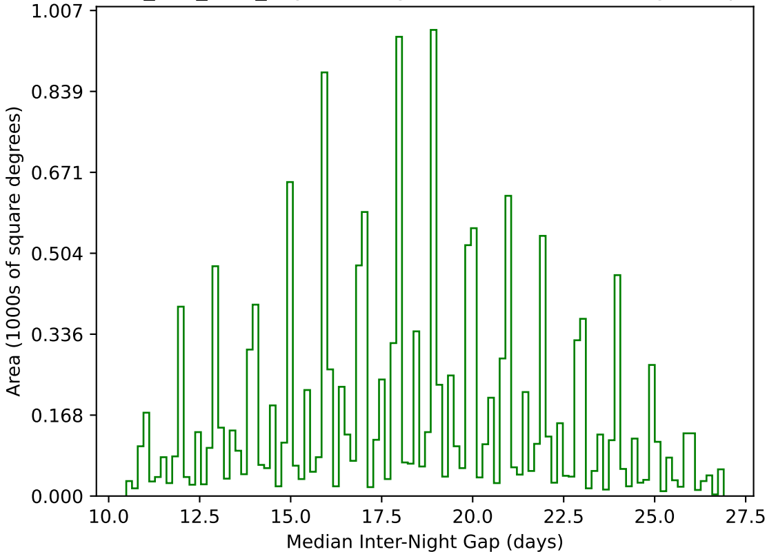
ddf_half_v3.4_10yrs WFD g band: Median Inter-Night Gap
