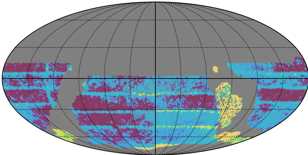
ddf_half_v3.4_10yrs WFD all bands: Median Inter-Night Gap
