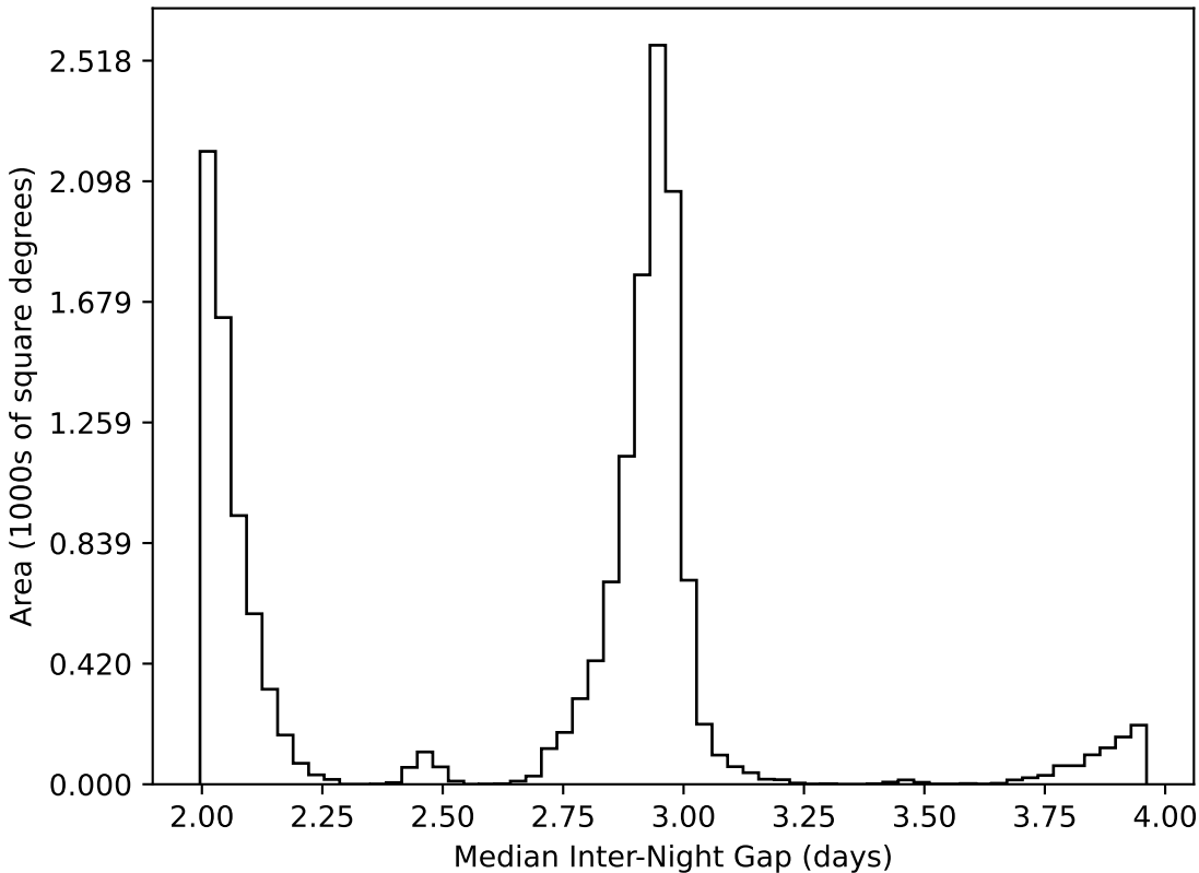
ddf_half_v3.4_10yrs WFD all bands: Median Inter-Night Gap
