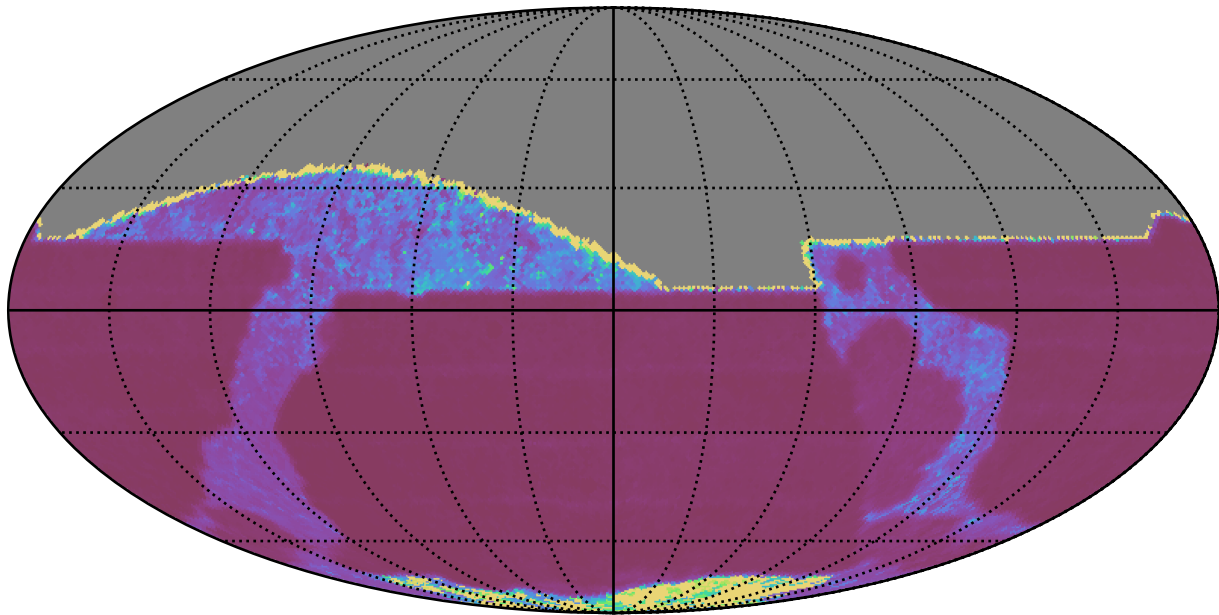
ddf_half_v3.4_10yrs All sky z band: Median Inter-Night Gap
