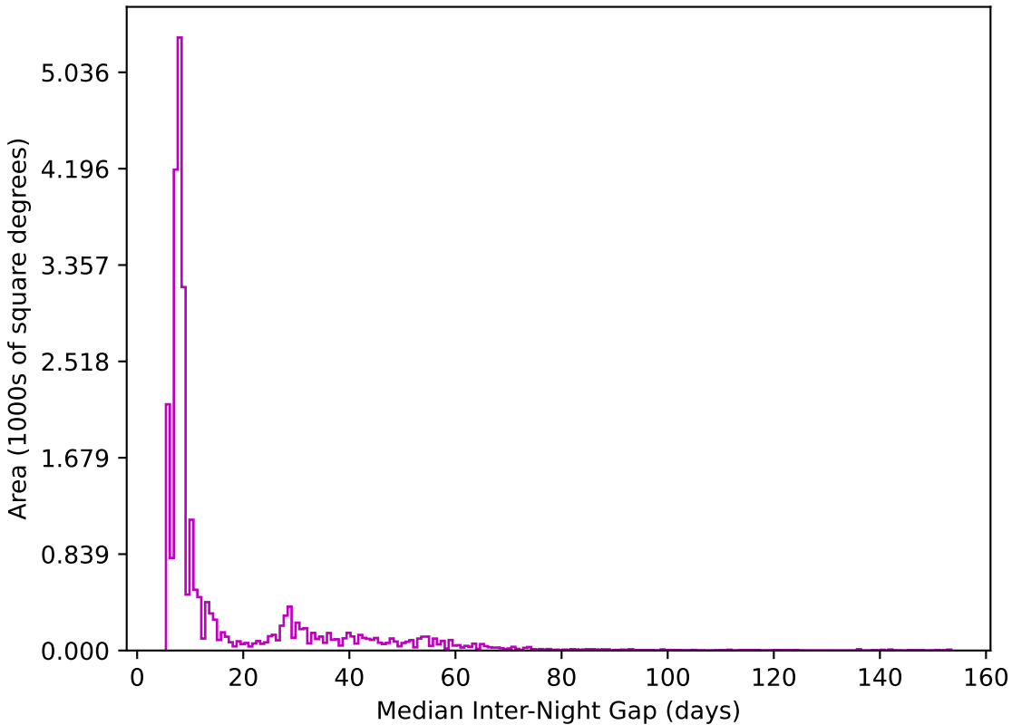
ddf_half_v3.4_10yrs All sky z band: Median Inter-Night Gap
