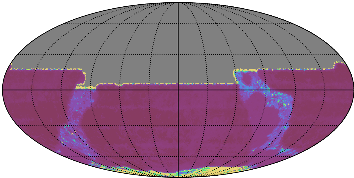
ddf_half_v3.4_10yrs All sky y band: Median Inter-Night Gap
