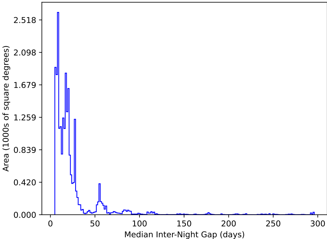
ddf_half_v3.4_10yrs All sky y band: Median Inter-Night Gap
