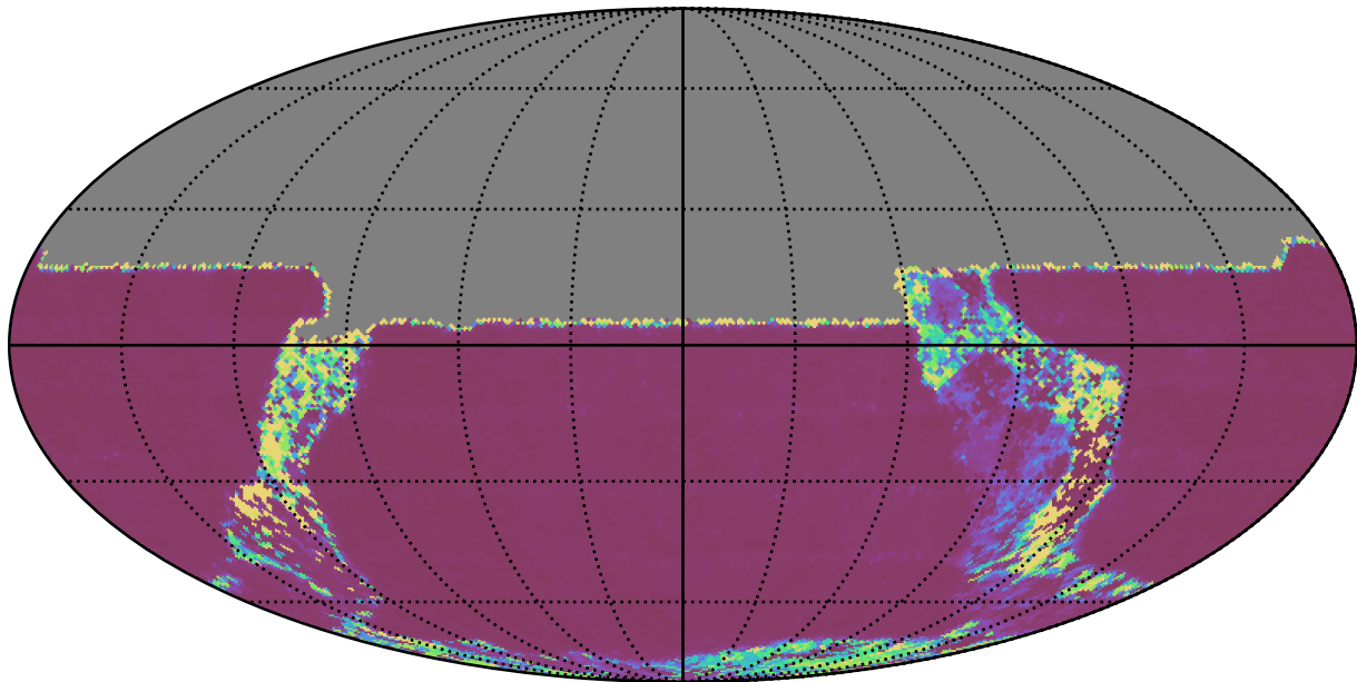
ddf_half_v3.4_10yrs All sky u band: Median Inter-Night Gap
