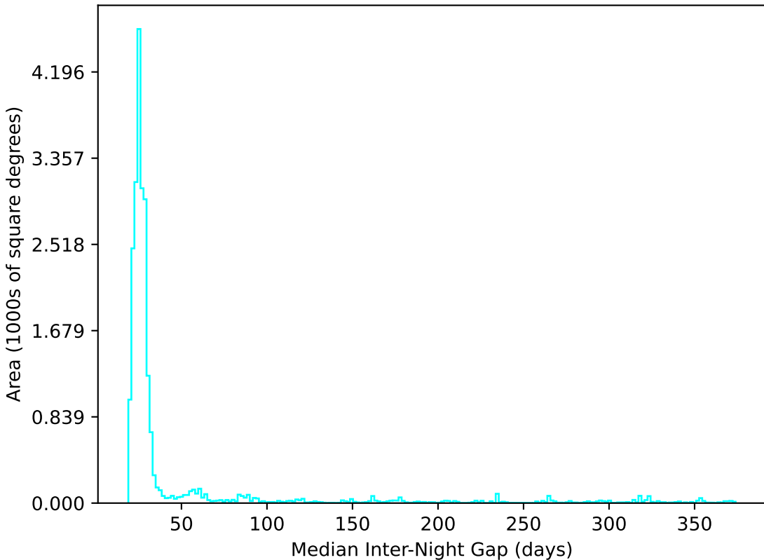
ddf_half_v3.4_10yrs All sky u band: Median Inter-Night Gap
