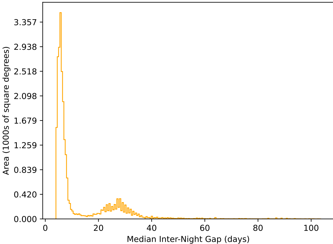
ddf_half_v3.4_10yrs All sky r band: Median Inter-Night Gap
