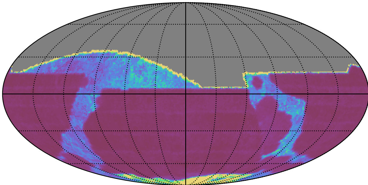
ddf_half_v3.4_10yrs All sky i band: Median Inter-Night Gap
