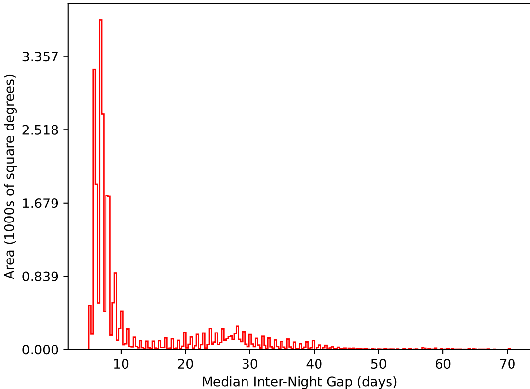
ddf_half_v3.4_10yrs All sky i band: Median Inter-Night Gap
