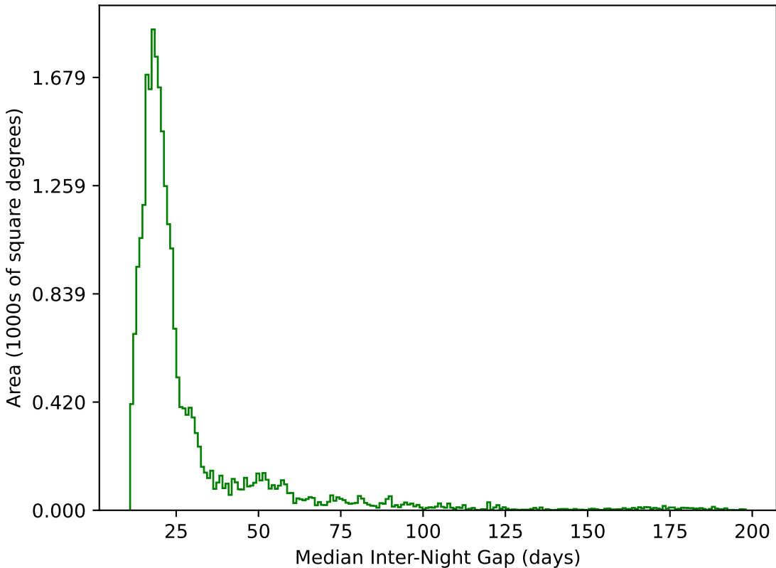
ddf_half_v3.4_10yrs All sky g band: Median Inter-Night Gap
