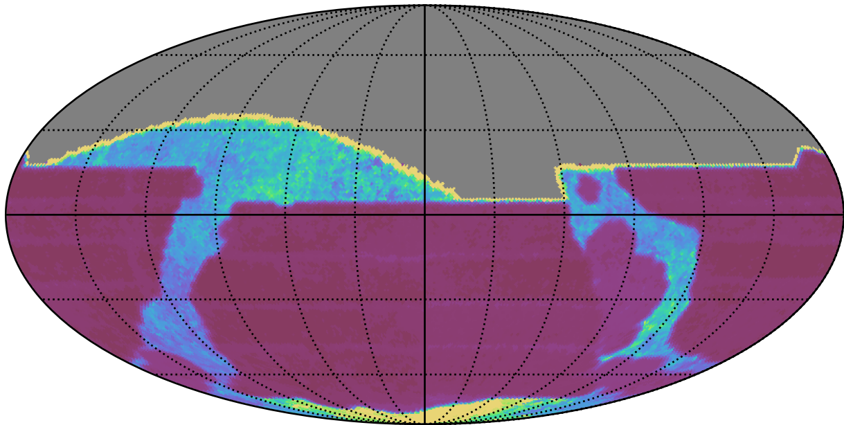
ddf_half_v3.4_10yrs All sky all bands: Median Inter-Night Gap
