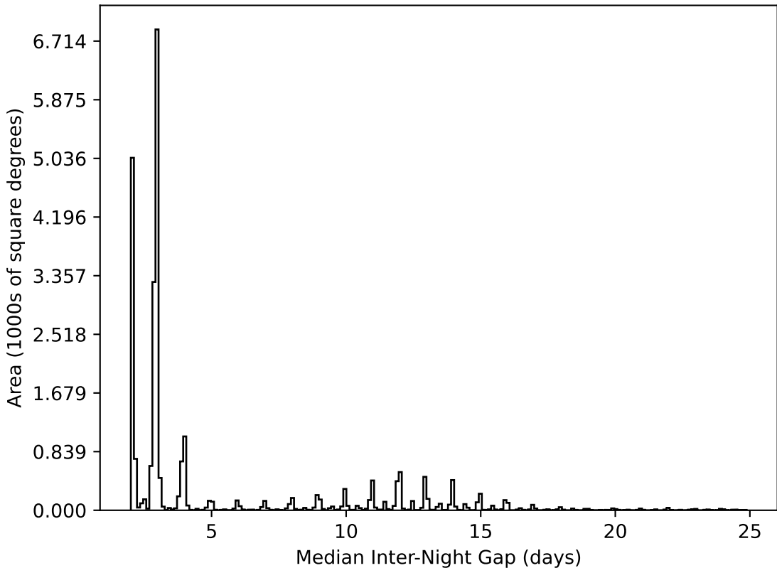
ddf_half_v3.4_10yrs All sky all bands: Median Inter-Night Gap
