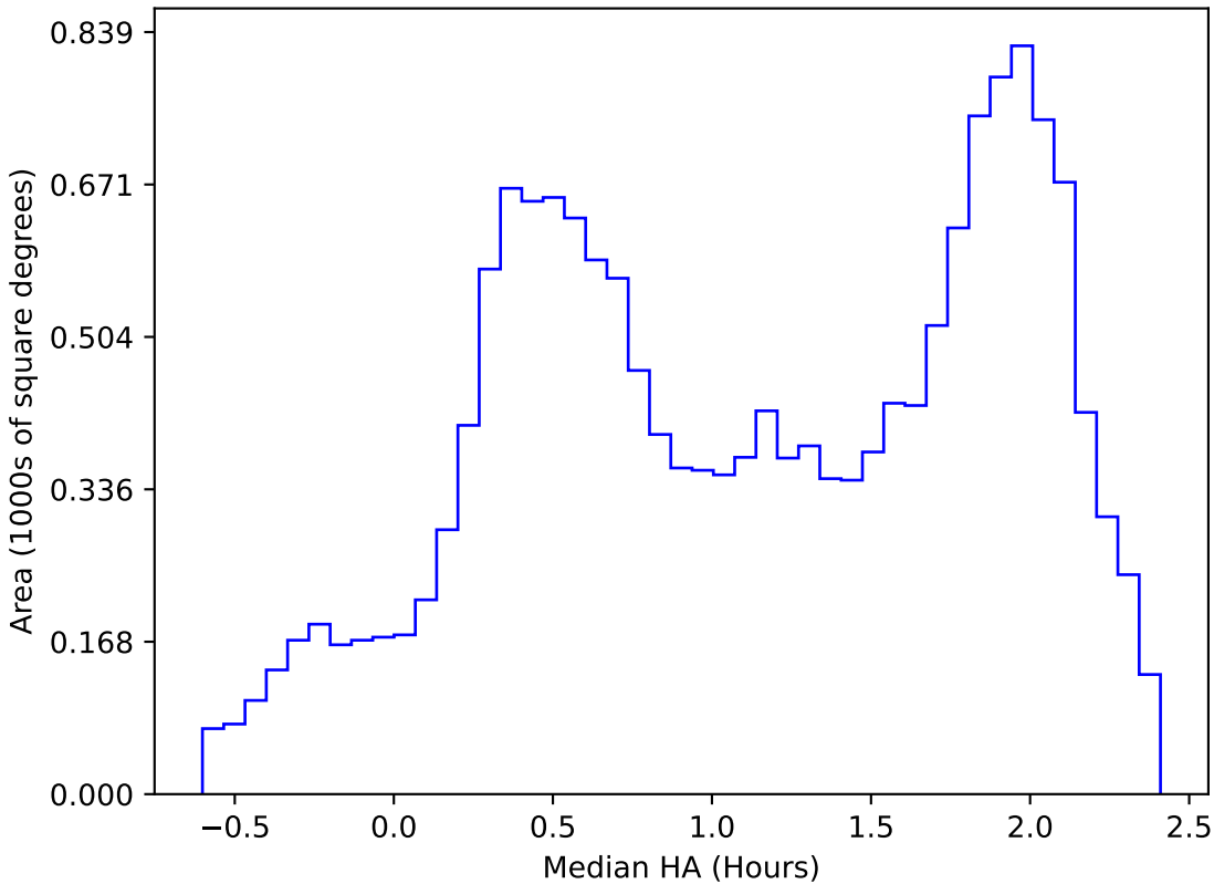
ddf_half_v3.4_10yrs WFD z band: Median HA
