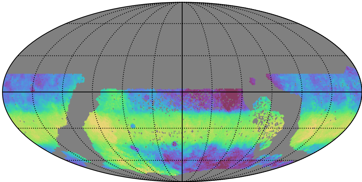
ddf_half_v3.4_10yrs WFD y band: Median HA
