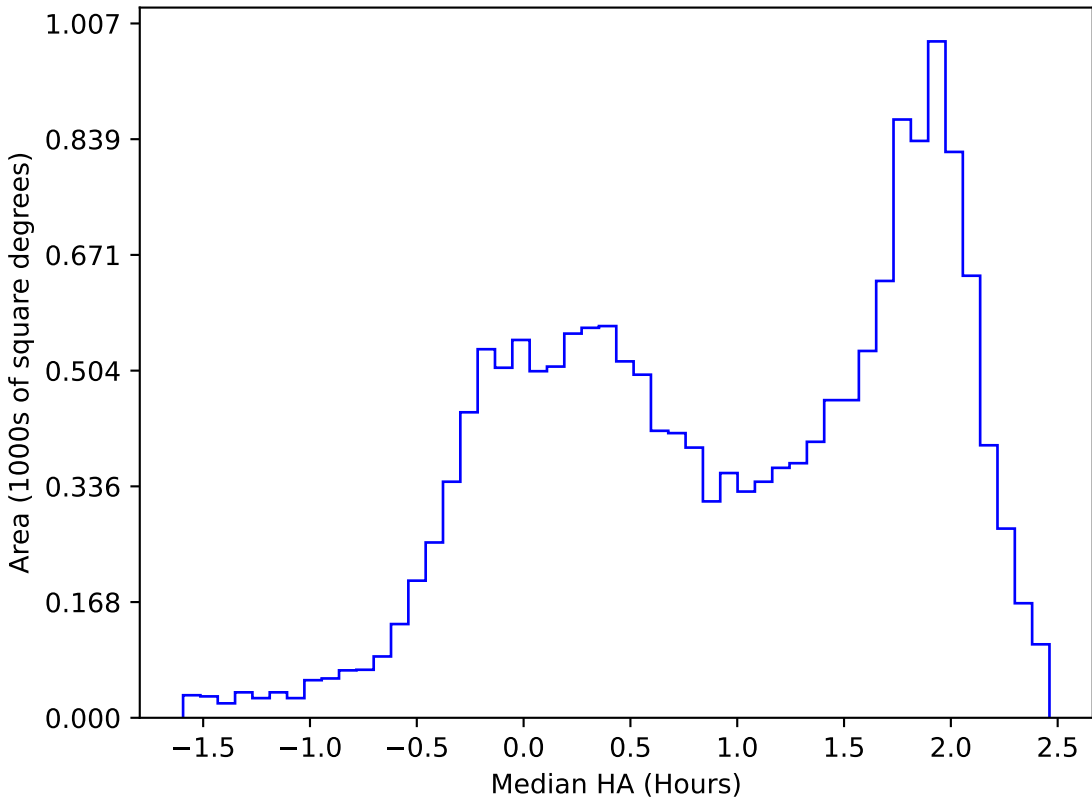
ddf_half_v3.4_10yrs WFD u band: Median HA
