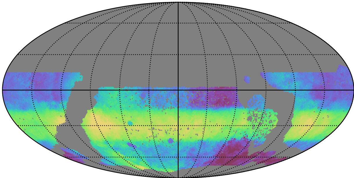
ddf_half_v3.4_10yrs WFD r band: Median HA
