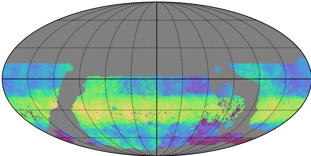
ddf_half_v3.4_10yrs WFD g band: Median HA
