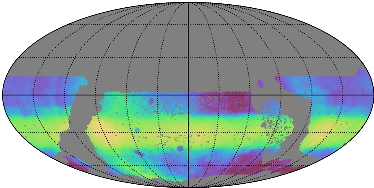
ddf_half_v3.4_10yrs WFD all bands: Median HA
