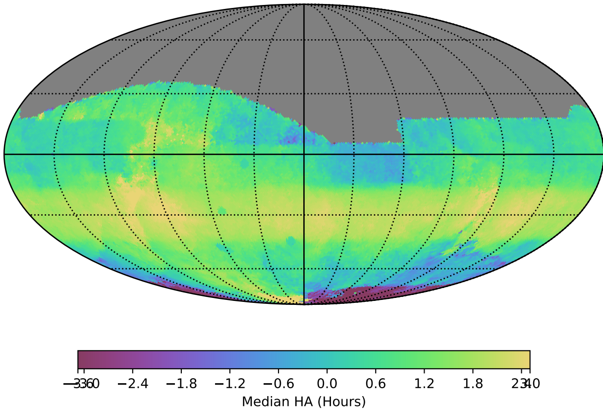
ddf_half_v3.4_10yrs All sky z band: Median HA
