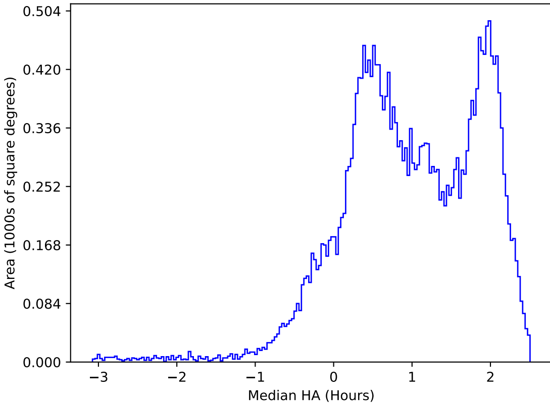
ddf_half_v3.4_10yrs All sky z band: Median HA
