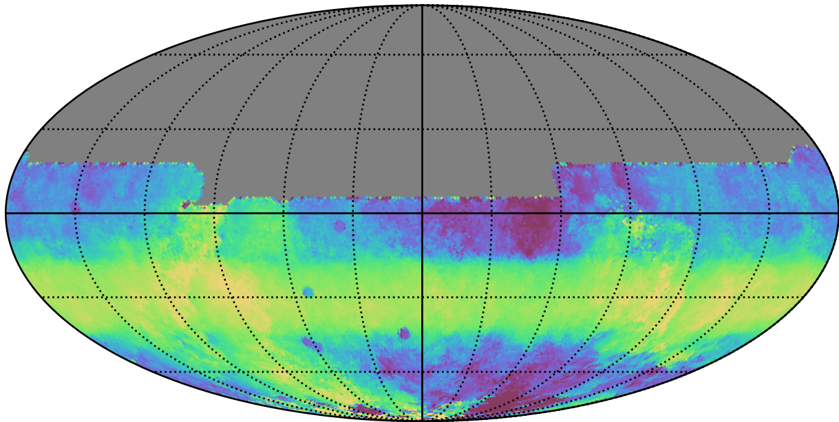
ddf_half_v3.4_10yrs All sky y band: Median HA
