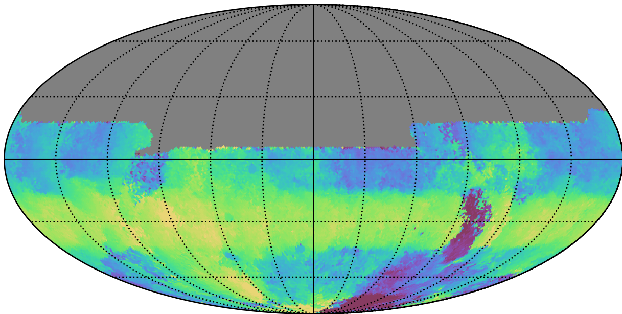
ddf_half_v3.4_10yrs All sky u band: Median HA
