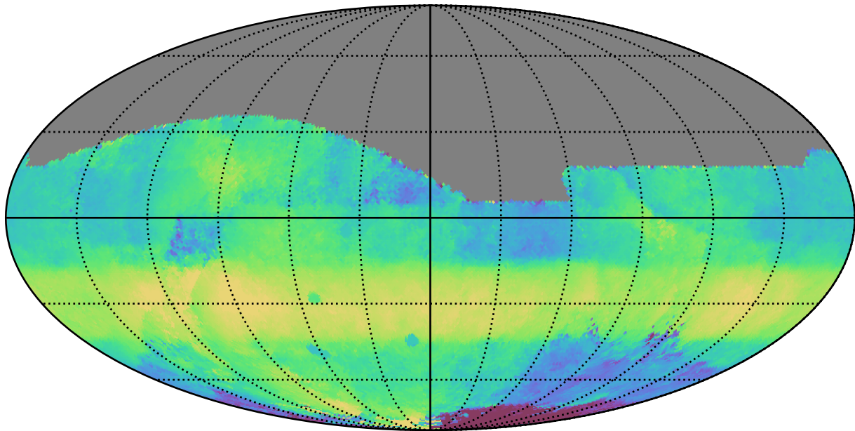
ddf_half_v3.4_10yrs All sky r band: Median HA
