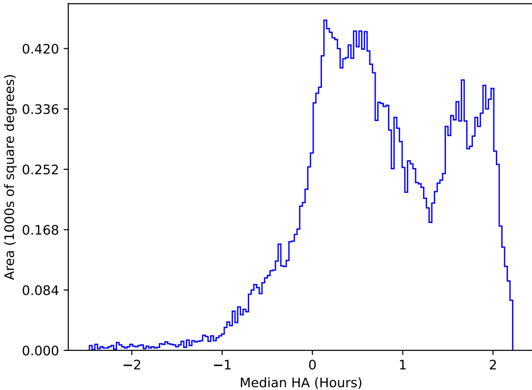
ddf_half_v3.4_10yrs All sky r band: Median HA
